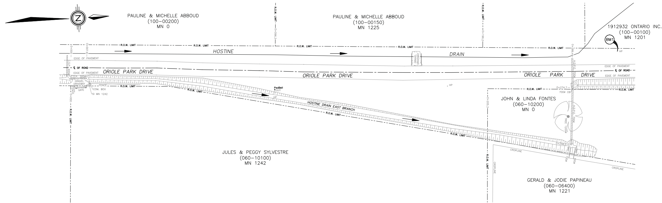
PLAN SCALE=1:500
