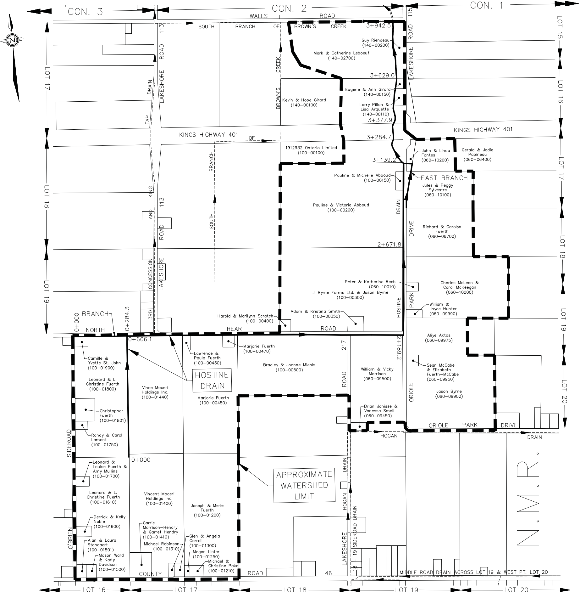
WATERSHED PLAN Scale = 1:6,000
