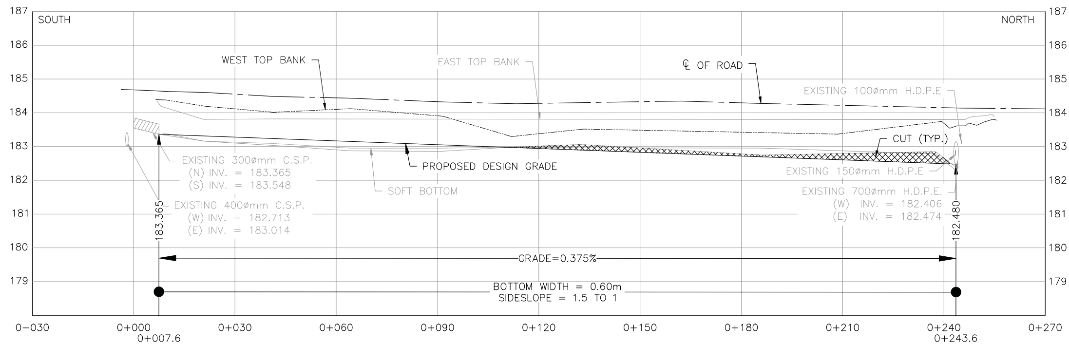
PROFILE SCALE H = 1:500 SCALE V = 1:50
