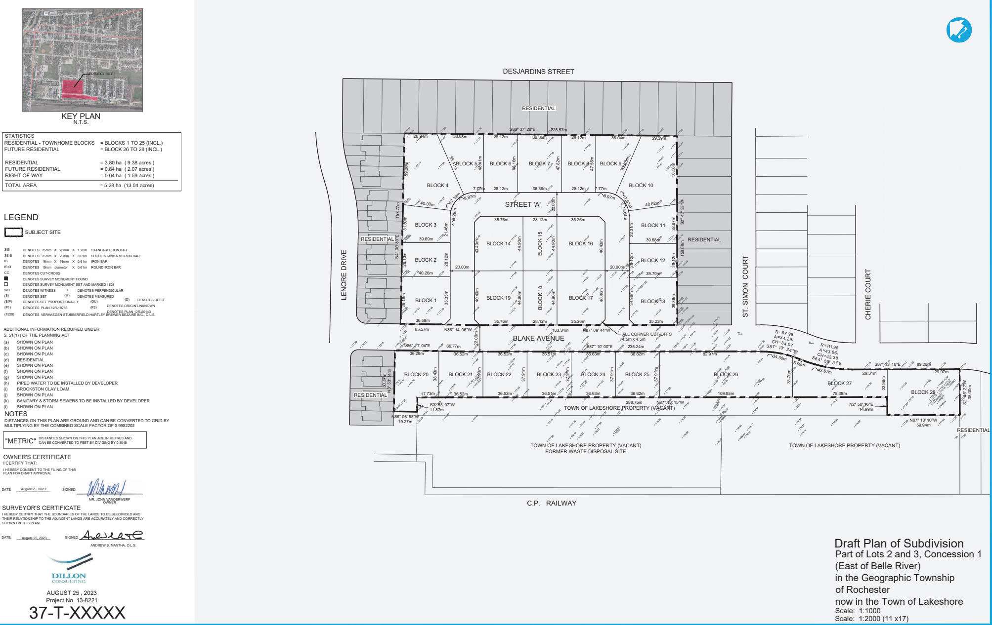
Figure 1.0 - Draft Plan of Subdivision, August 25, 2023
