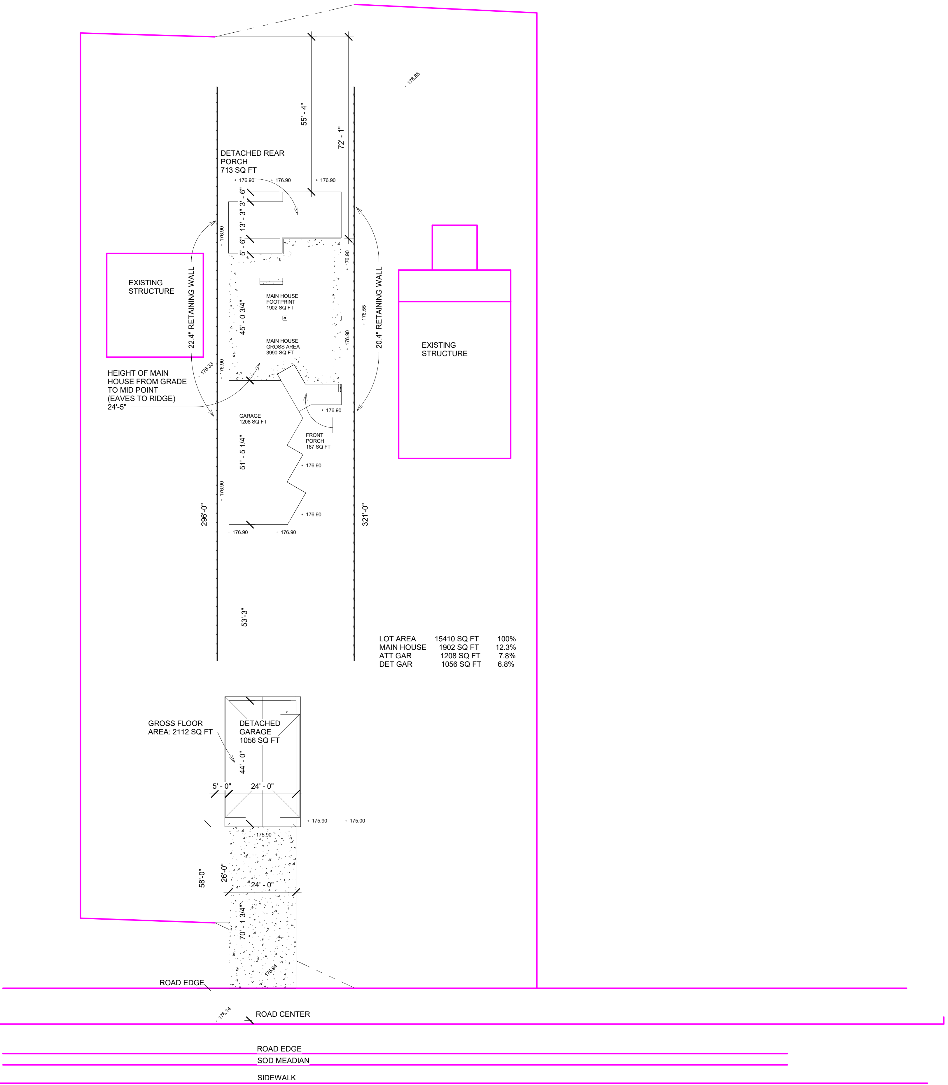
1 Site Plan 1" = 20'-0"
